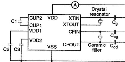
Figure 5. Supply current measurement 2
