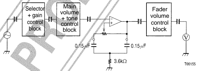
Treble Characteristics
