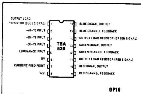
Fig. 1 Pin connections
